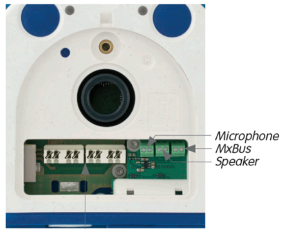
Ethernet installation cable LSA terminal block
